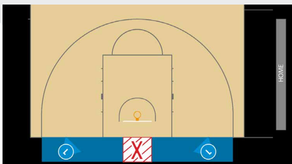
Diagram 27: Lead working area is between 3 point line and edge of the board. To find out if you have the correct position is to check that you will see the front of the rim.
